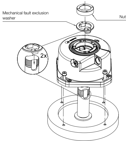
Front end shaft coupling with pins
