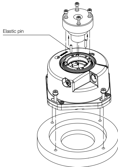
Front end shaft coupling with pins
